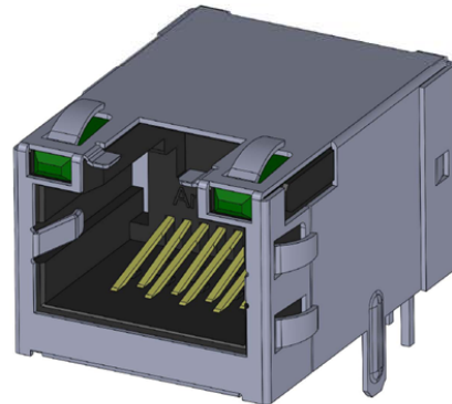
P/N RJE48-188-1XX1 SHOWN SINGLE PORT, 8 POSITION, WITH SHIELD AND LEDs
